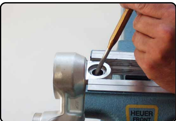
Tap the other adaptor bush out of the heim-joint.
